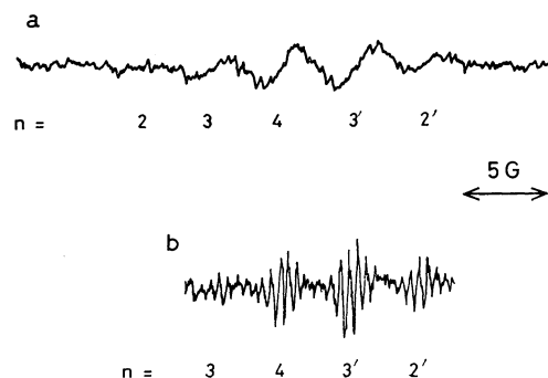
Fig. 3. ESR spectra of durosemiquinone radical DQH· in i -PrOH at 260 K.
